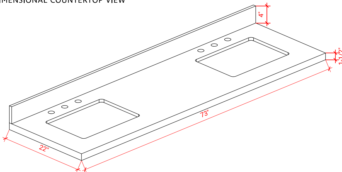
THREE DIMENSIONAL COUNTERTOP VIEW
