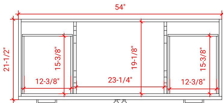
PLAN VIEW
