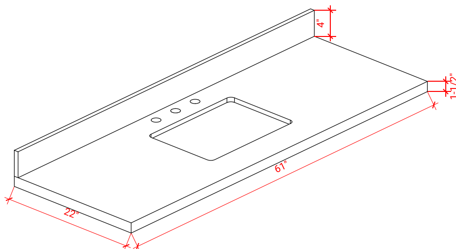
THREE DIMENSIONAL COUNTERTOP VIEW
